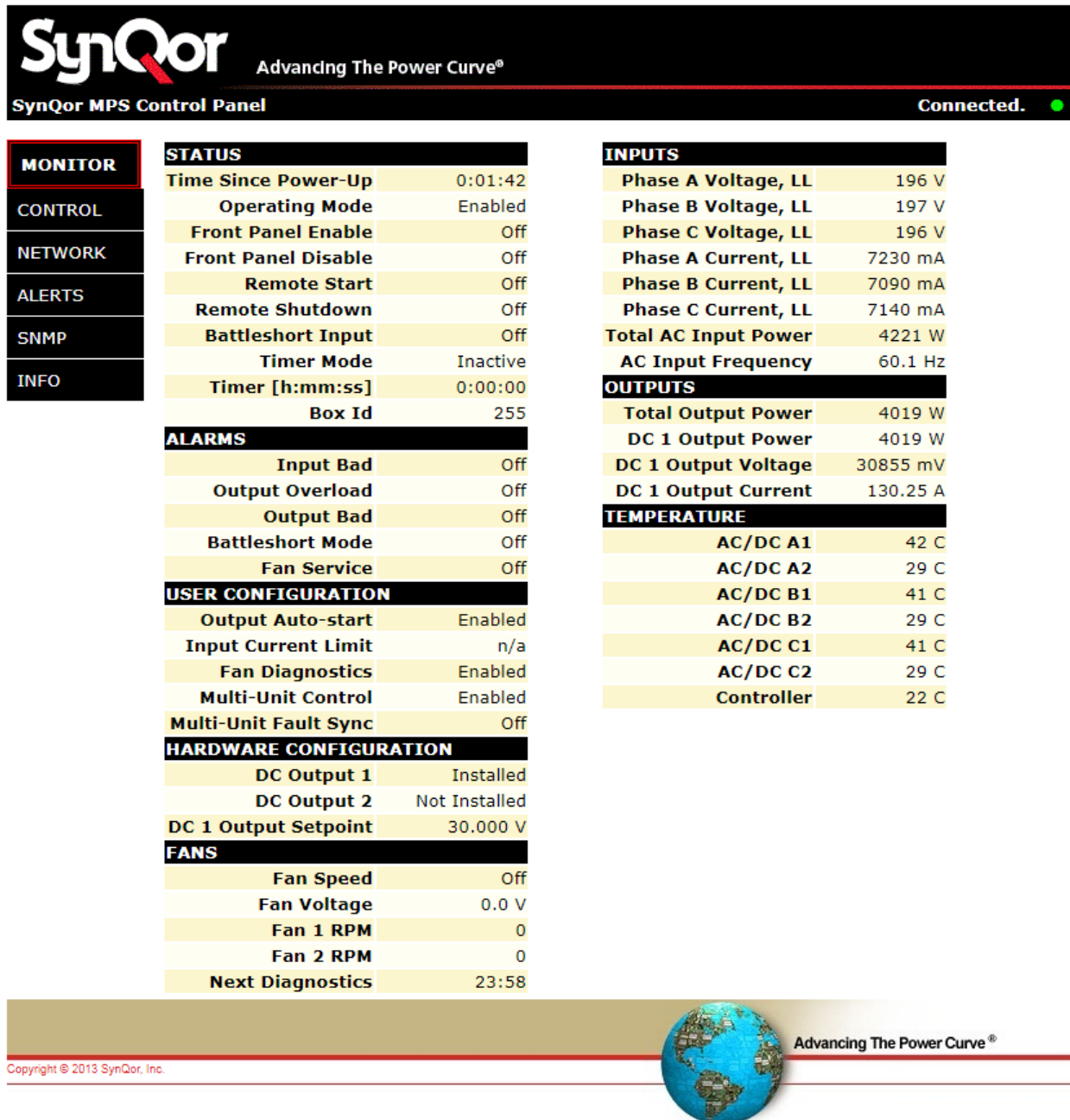
Figure A Monitor Page of Web Interface
